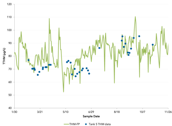
Figure 3- THM-FP data predicting THM levels at an endpoint of the GHWTP’s distribution system.
