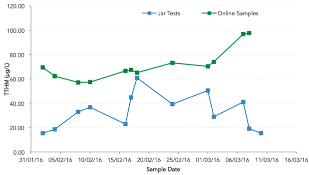
Figure 2- Chlorine Dioxide Jar Test THM Results Compared to GHWTP Finished Water - 13 jar tests/month, 6 bottles/jar test, 78 samples/month.
