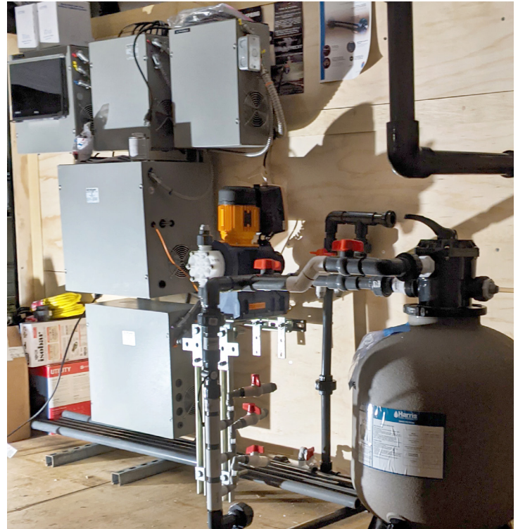
SafeGuard H2O trailer-mounted arsenic removal demonstration system installed at Isleton Well #3A.
