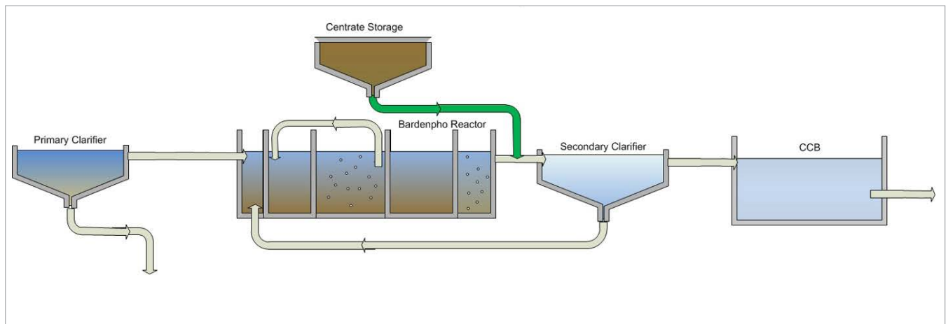
Centrate Process Diagram
